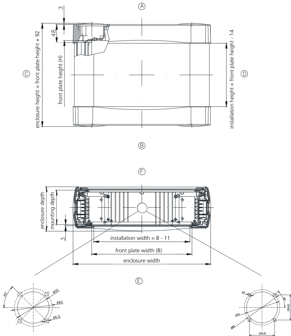
Drilling hole GT 48/2 and GTK electronic
