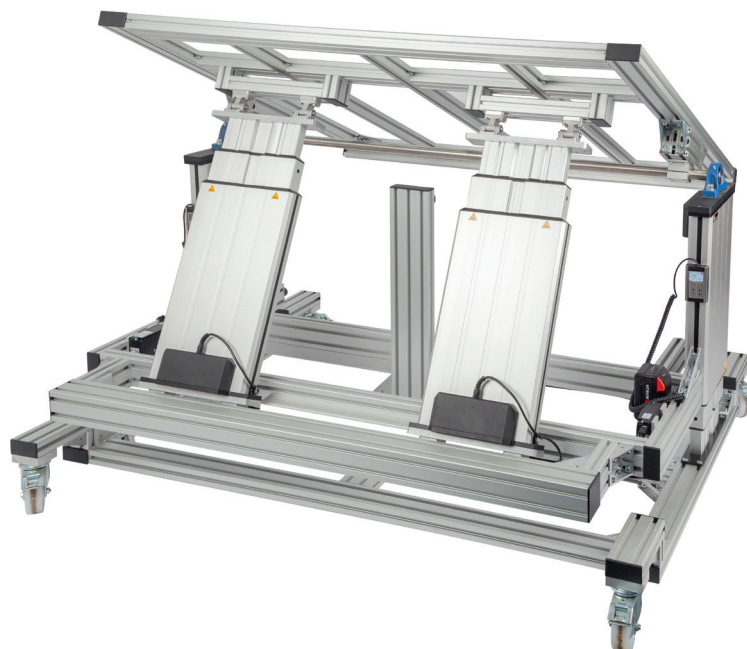
RK Easymount 300
