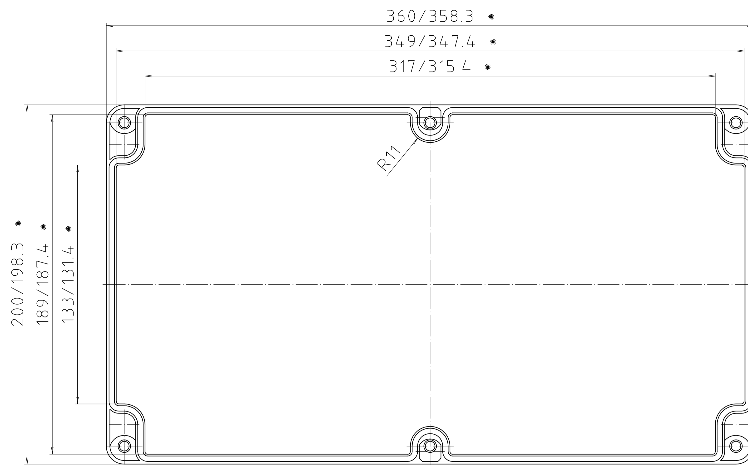
Deckel/lid
