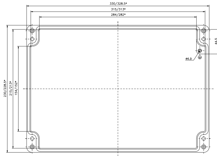
Deckel
