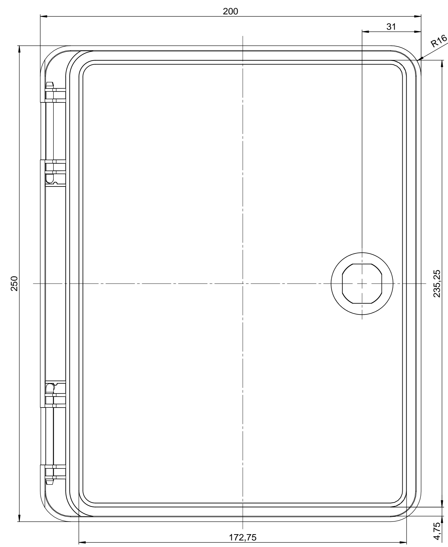
Deckel
