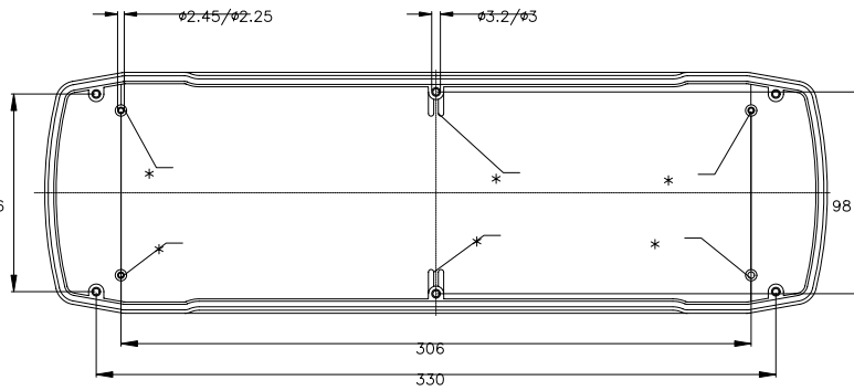
Oberschale/enclosure top
