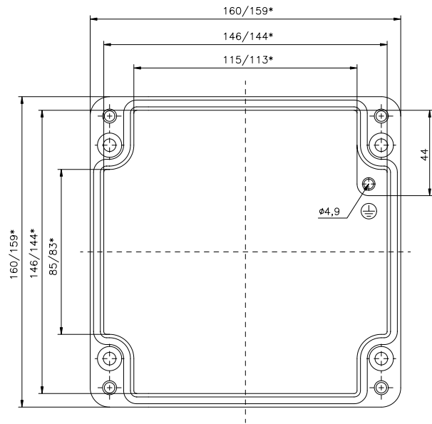
Deckel
